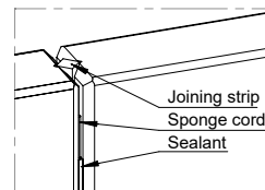
Element connection
