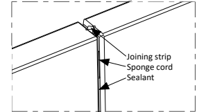
Element connection
